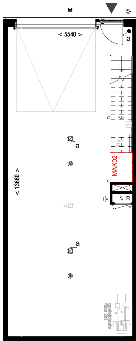
Begane grond, PEIL=0
