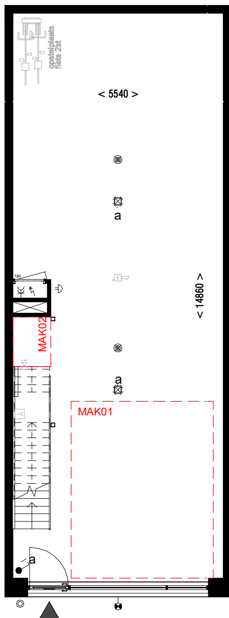
Begane grond, PEIL=0
